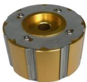
100W Flat Type Cutter Body Part Code HE100WB Dimension 100x \phi 160
